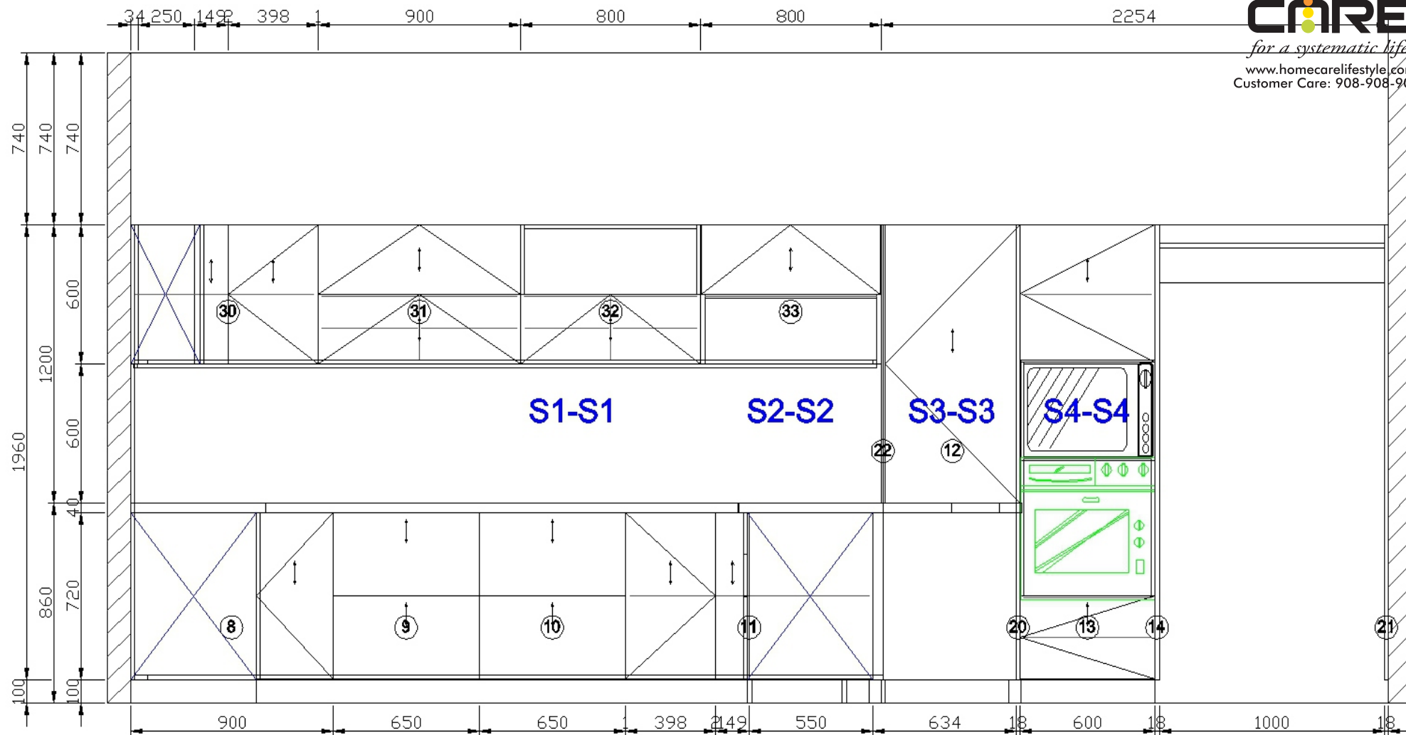
C View elevation drawing
