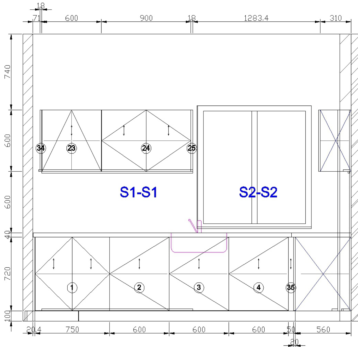
A View elevation drawing
